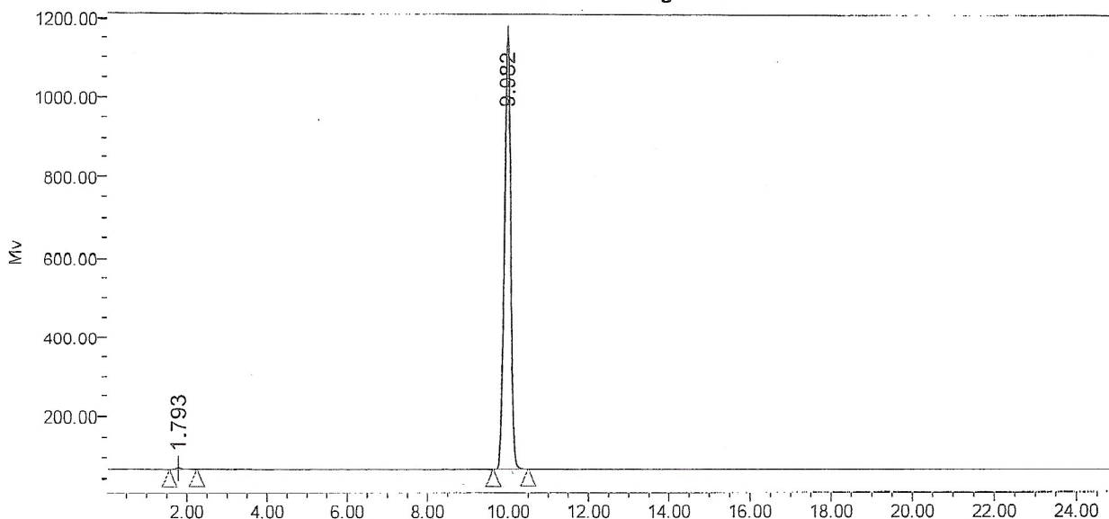
Auto-Scaled Chromatogram
